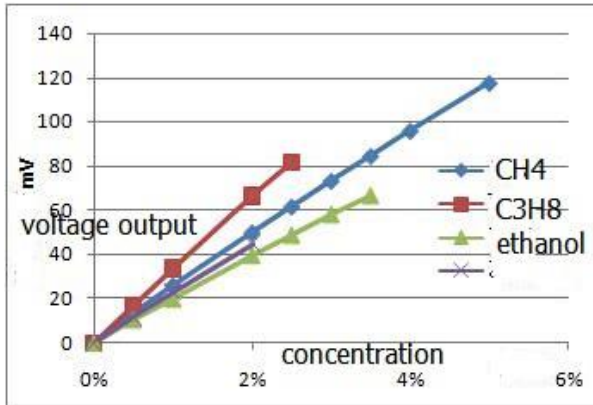
Fig3. Sensitivity Curve
