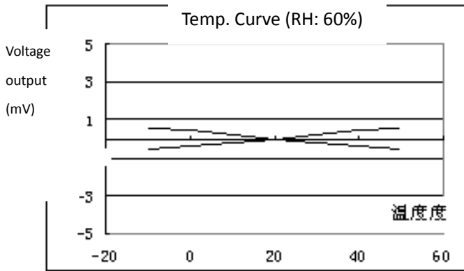
Fig5. Zero point at different temp.
