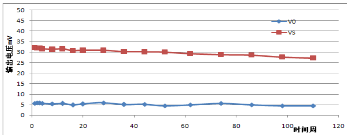
Fig11. Sensitivity fluctuation
