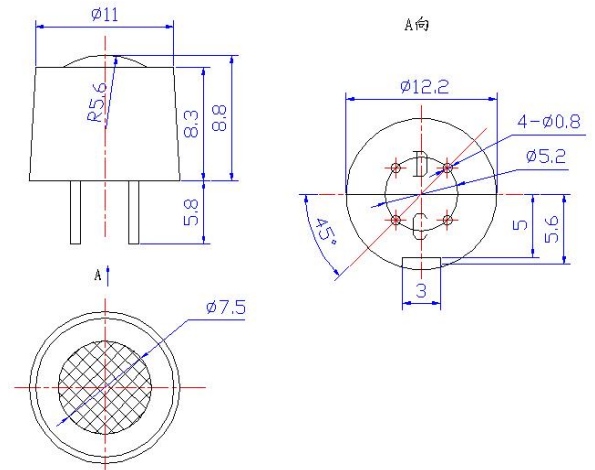
Fig1.Sensor Structure
