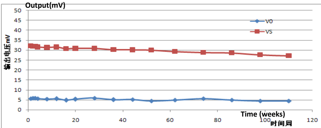
Fig10. Sensitivity fluctuation
