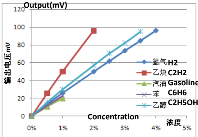
Fig3. Sensitivity Curve
