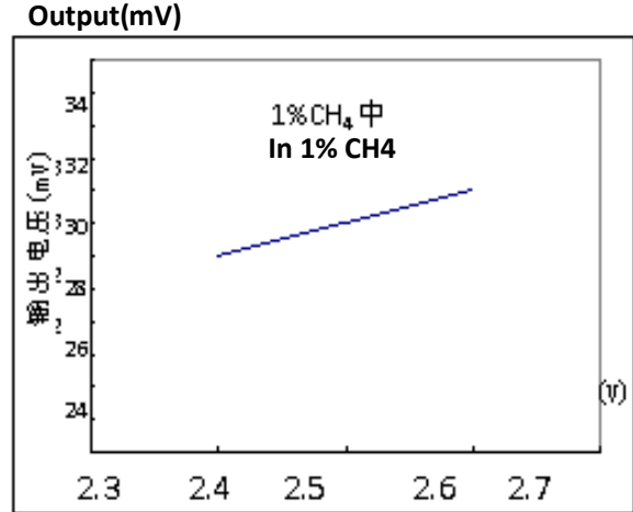
Fig9. Sensitivity with different voltage
