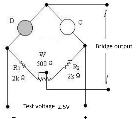
Fig1.Sensor Structure
