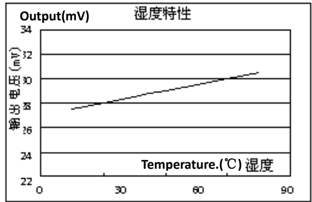
Fig5. Sensitivity at different temp.
