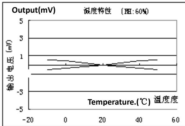
Fig5. Zero point at different temp.
