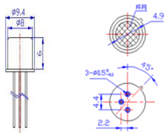
Fig1.Sensor Structure
