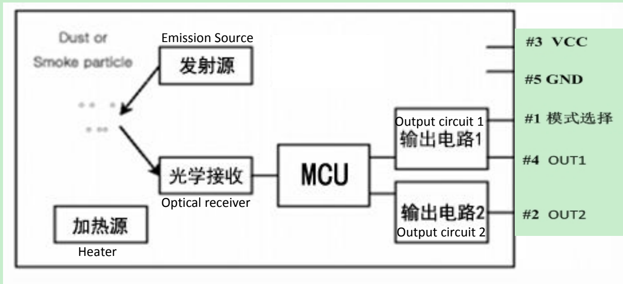
Fig 3.Principle schematic 2
