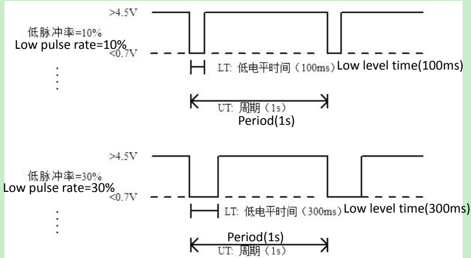
Fig5.PM2.5 output wave in PWM mode
