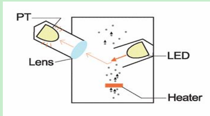
Fig 2.Principle schematic 1
