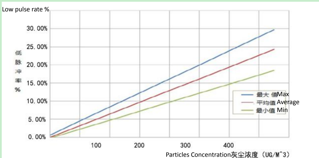
Fig7.The relationship of PM2.5 low pulse rate of output and dust particles concentration
