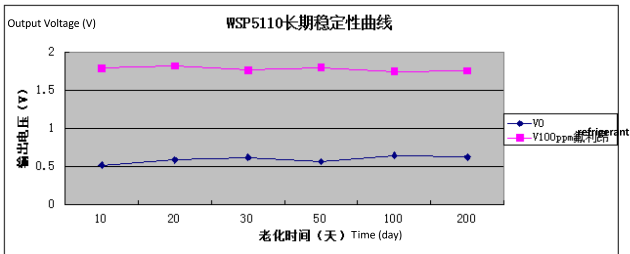
Fig7.long-term Stability
