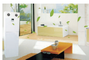
Smart Home
