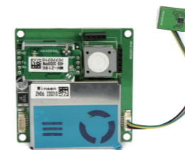
ZPHS01C-Formaldehyde Version (CO 2 , PM2.5/10, CH 2 O, T&H)
