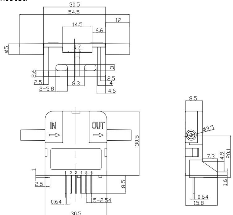
Fig1. Sensor Structure
