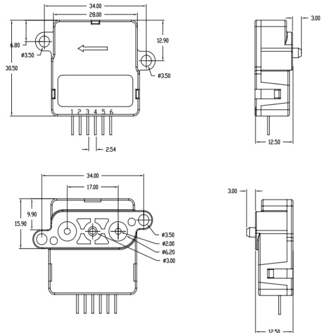
Fig1.Sensor Structure
