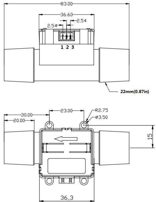
Fig1. Sensor Structure
