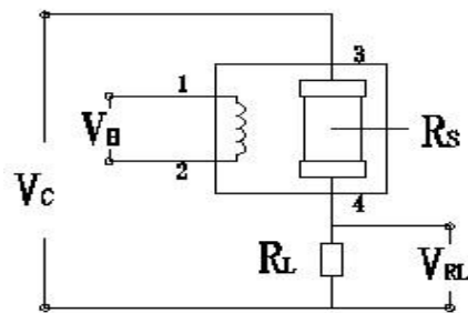
Fig2. WSP5110 Test Circuit
