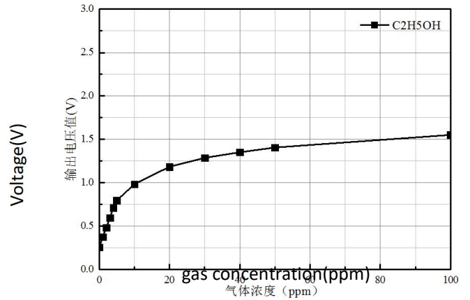
Fig6. Linearity character
