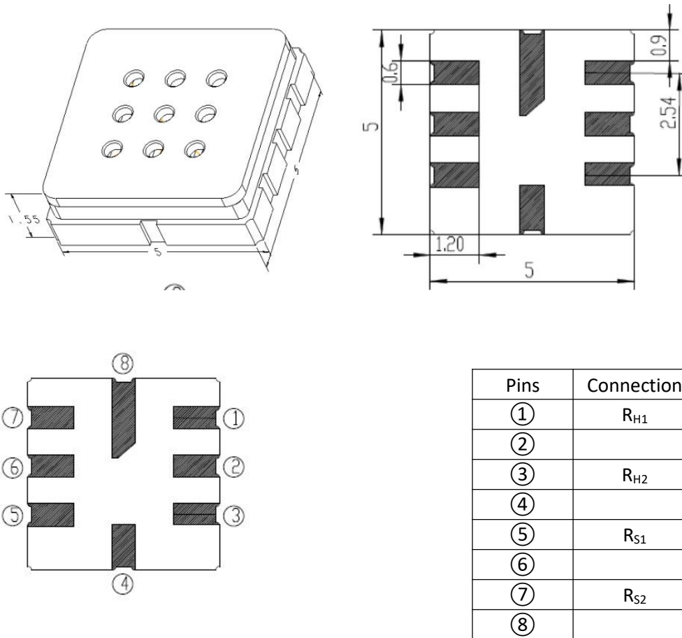
Fig1. Sensor structure
