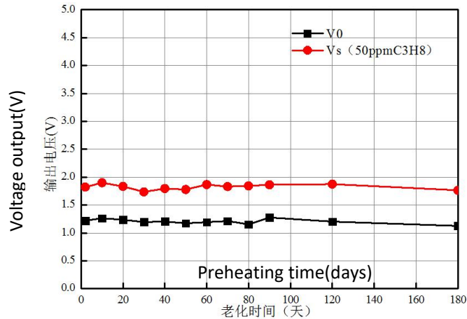
Fig7.long-term Stability
