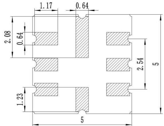
Bottom view (unit:mm)
