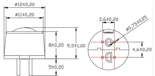
Fig1. Sensor Structure
