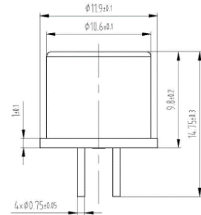
Fig1. Sensor Structure Tolerance ±0.1mm
