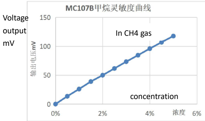
Fig3.Sensitivity Curve
