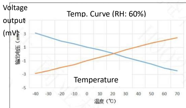
Fig5.Zero point at different temp.
