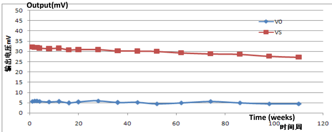
Fig11. Sensitivity fluctuation
