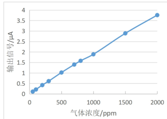
Fig4. Linearity curve
