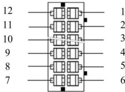
Figure 2: Pin Definition
