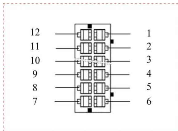
Figure 2 Pin Definition
