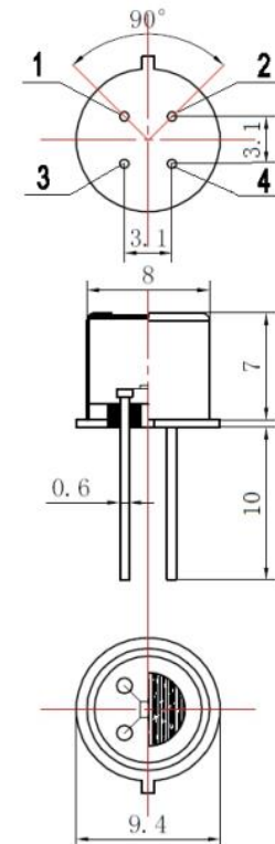
Fig1. Sensor structure
