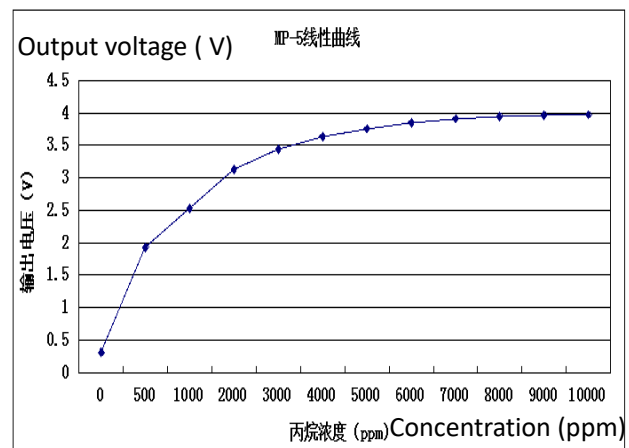
Fig6. Linearity curve
