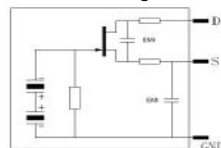
Component Structure Basic Testing Circuits
