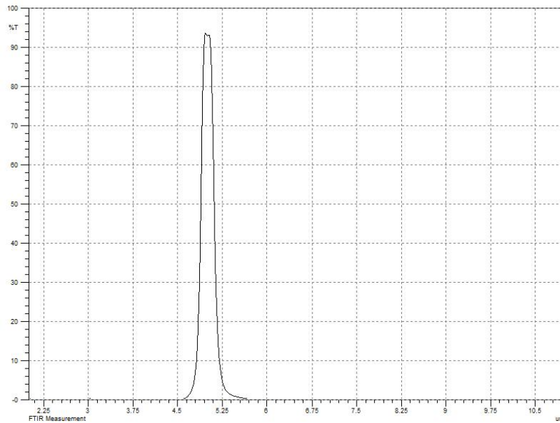
5.0µm narrow band filter spectral curve
