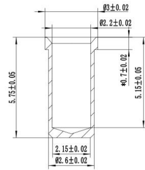
Picture 2: Tube base dimensions
