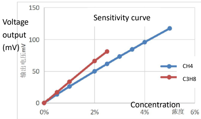
Fig3. Sensitivity Curve
