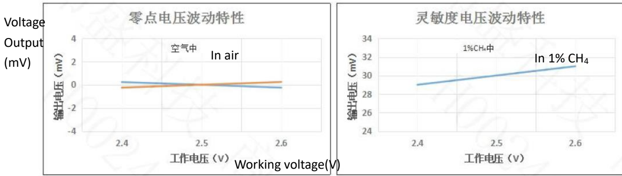
Fig9.Zero Drift with different voltage
