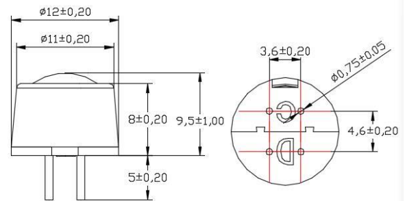
Fig1. Sensor Structure
