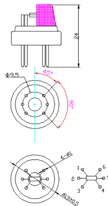
Fig1.Sensor Structure
