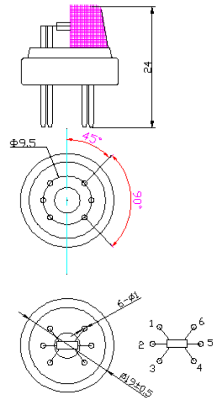
Fig1.Sensor Structure
