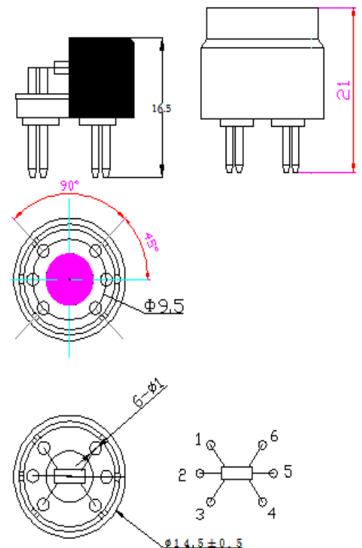
Fig1.Sensor Structure
