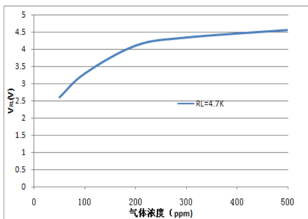
Fig5.Sensitivity Curve
