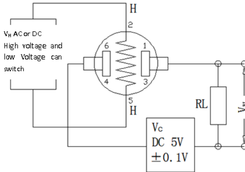
Fig2. MQ-9B Test Circuit
