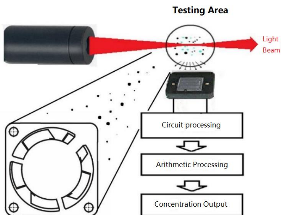
Fig3. Working principle
