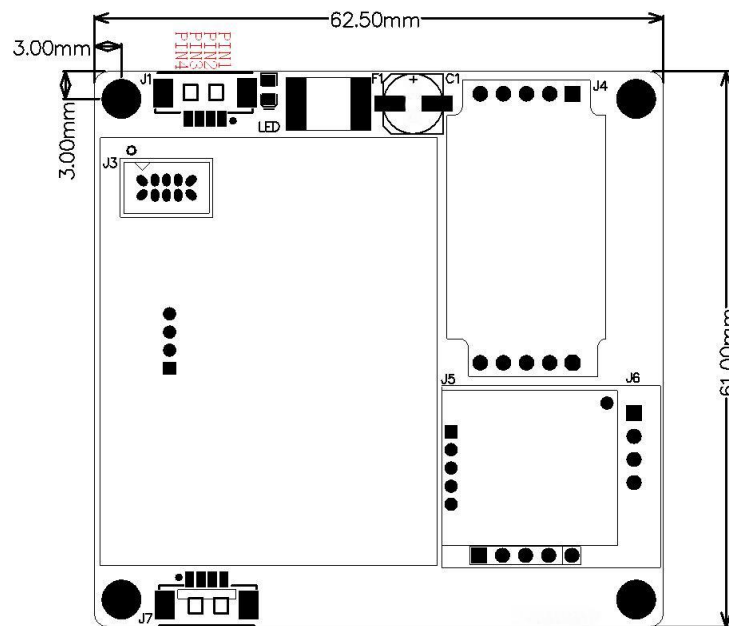
Fig 3: Mounting dimension
